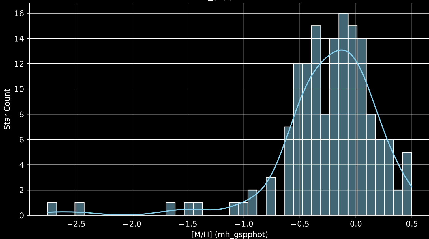
APOGEE DR17 Field: [TRIAND-5 [M/H] (mh_gspphot) (n= 152)
