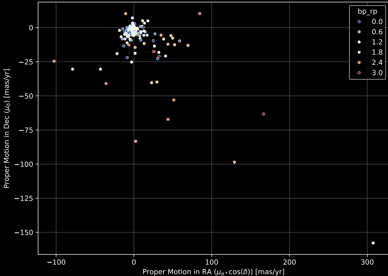
APOGEE DR17 Field: [TRIAND-5] Proper Motion Diagram (n= 153)
