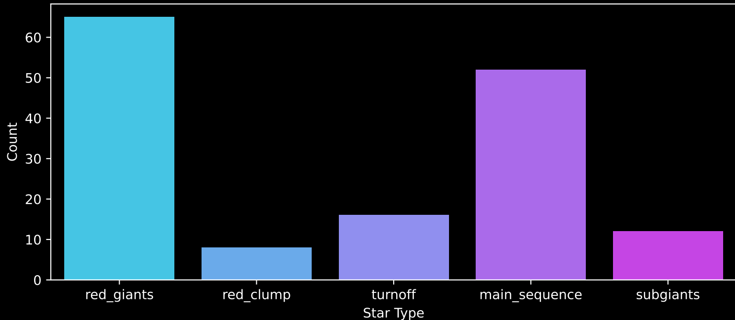
APOGEE DR17 Field: [TRIAND-5] Count plot of Star Type
