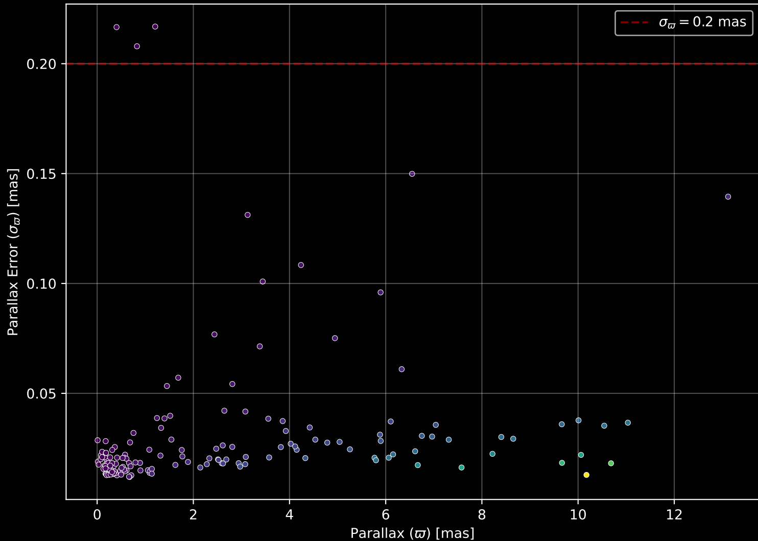
APOGEE DR17 Field: [TRIAND-5] Parallax Quality (n= 153)
