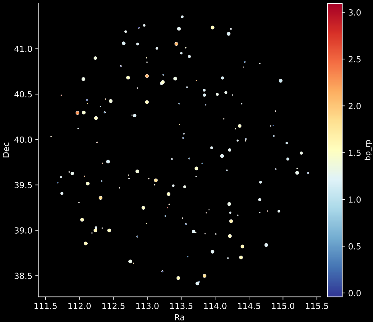
APOGEE DR17 Field: [TRIAND-5] Stars: 153
