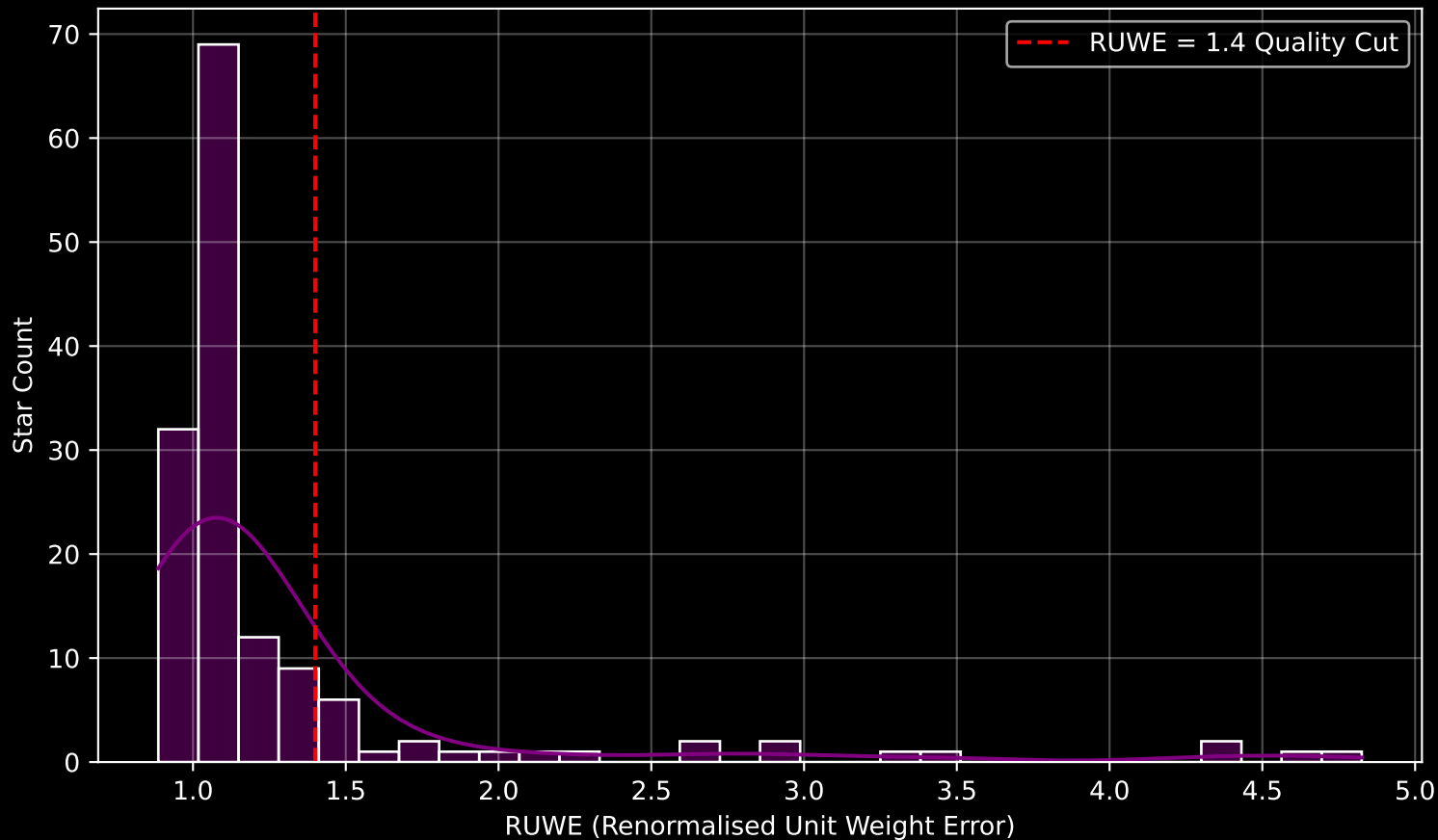
GAPOGEE DR17 Field [TRIAND-5] RUWE Distribution (n= 145)
